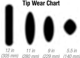
Tip Wear Chart
